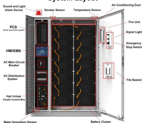
System Layout
